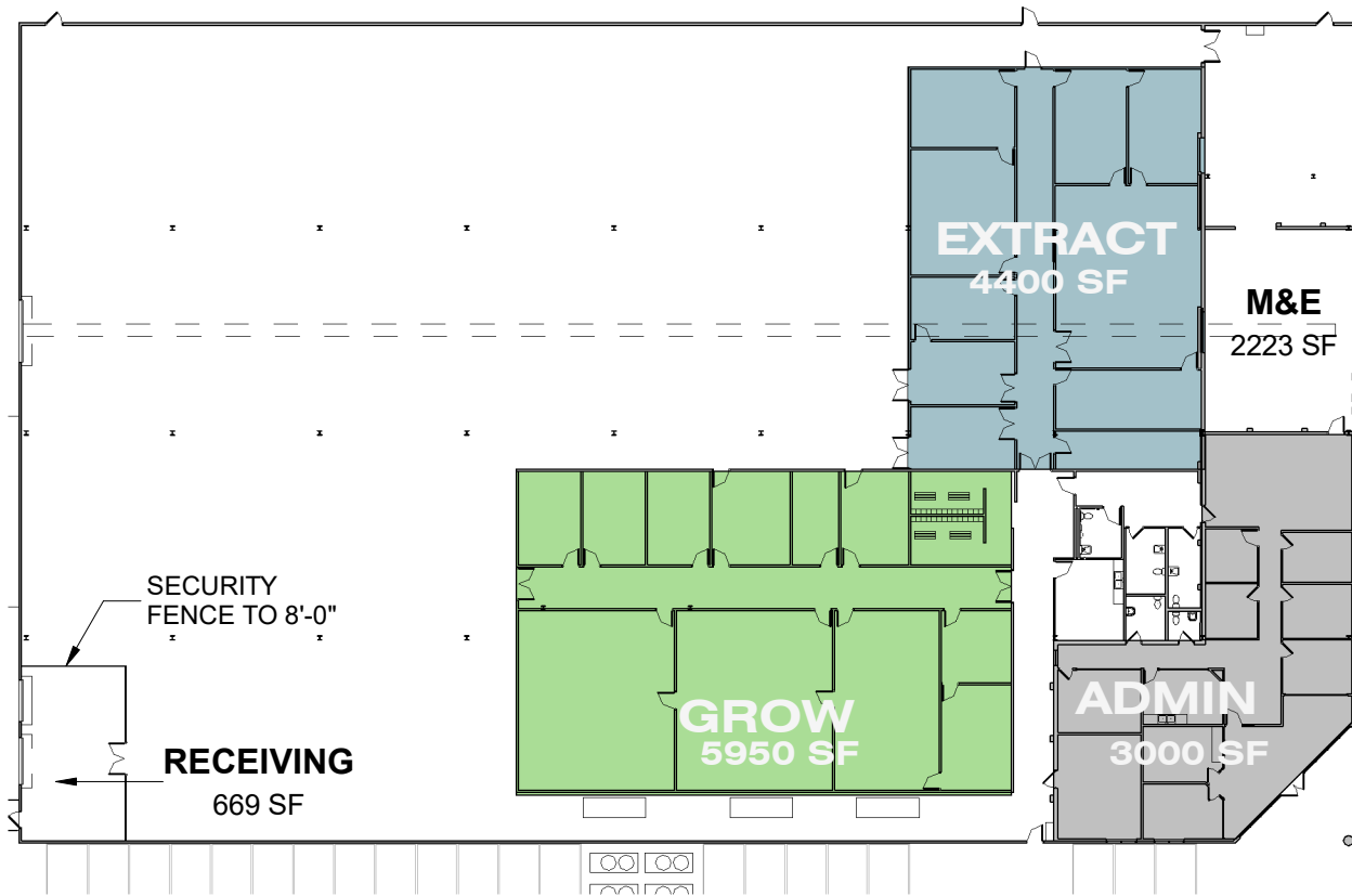
1 OVERALL CONSTRUCTION PLAN SCALE: 1" = 40'-0"
